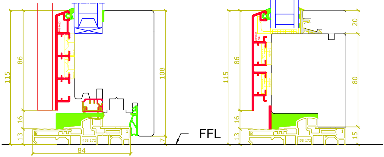
Openable section
